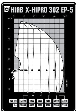
HIAB X-HIPRO 302 EP-5
