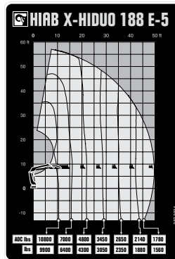
HIAB X-HIDUO 188E-5
