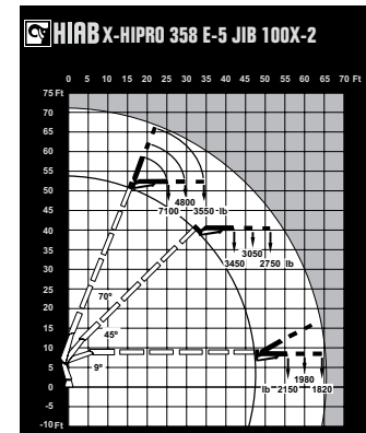
HIAB X-HIPRO 358E-5 JIB 100X-2
