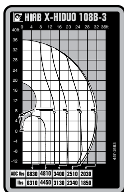
HIAB X-HIDUO 108B-3
