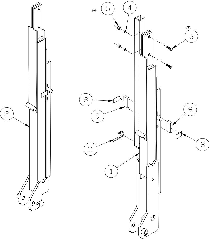
RUNNERS FOR SINGLE PIECE PLATFORMS
