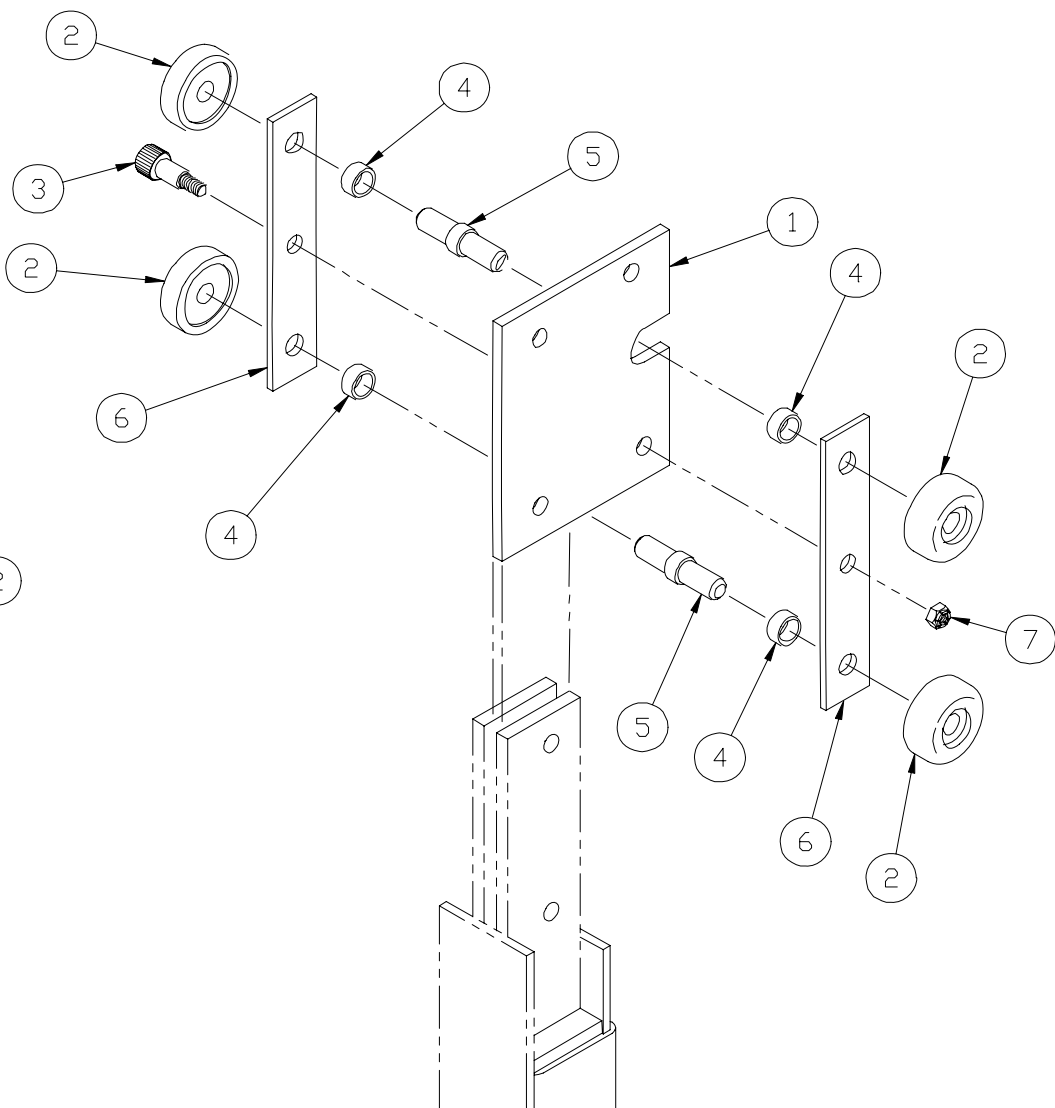
RGL-30, 40, 50, 60 UPPER TANDEM ROLLER ASSEMBLY COMPLETE
