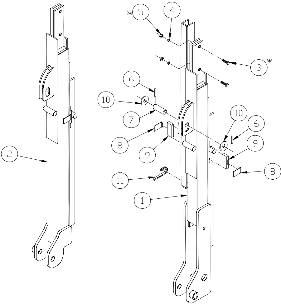
RUNNERS FOR TWO PIECE PLATFORMS
