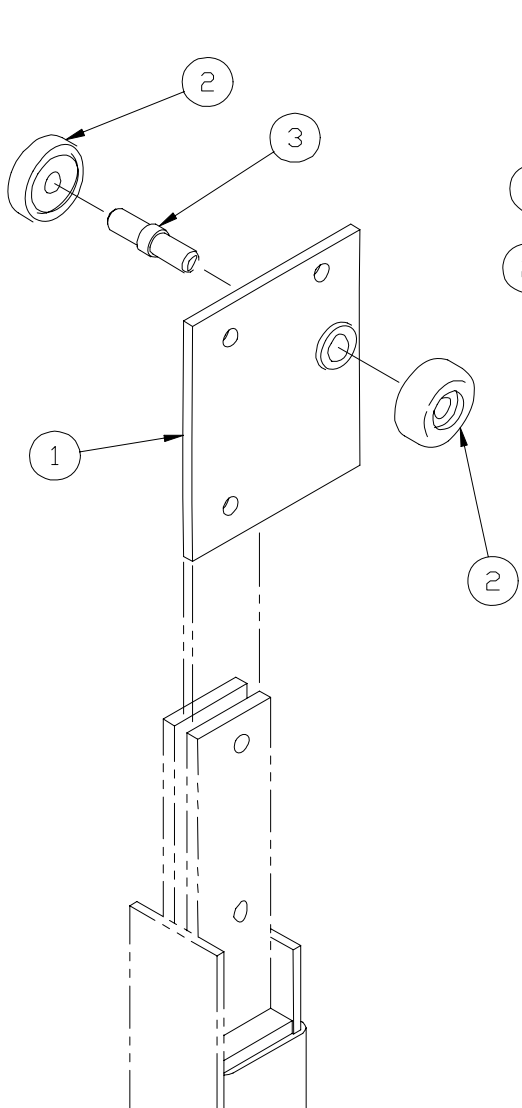
RGL-20 UPPER ROLLER ASSEMBLY COMPLETE
