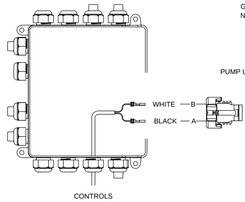
2- POLE CONNECTOR
