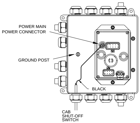
MAIN POWER CONNECTIONS
