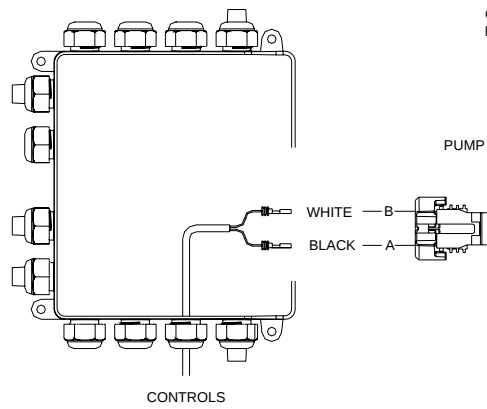
2- POLE CONNECTOR
