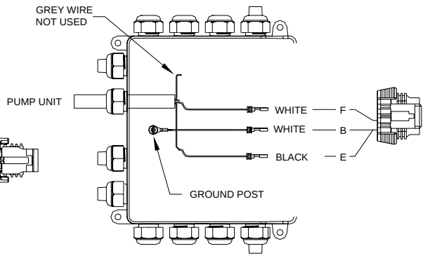
8- POLE CONNECTOR
