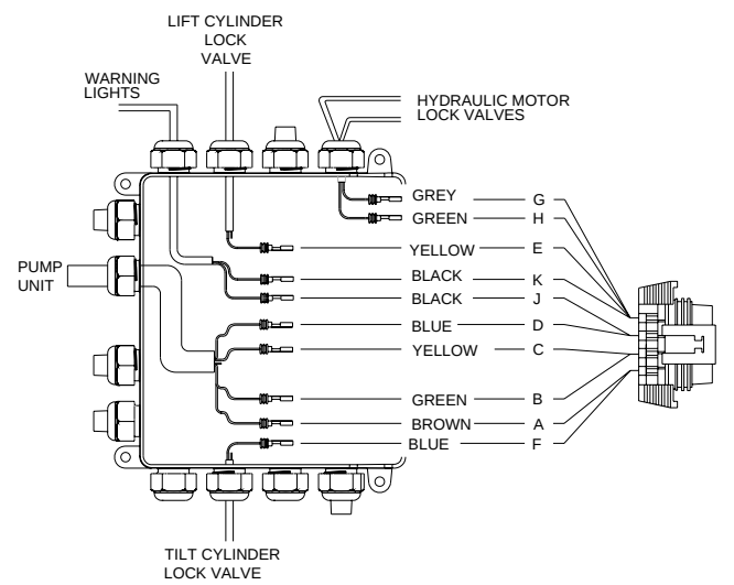
10- POLE CONNECTOR
