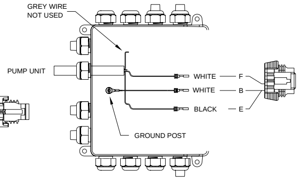
8- POLE CONNECTOR
