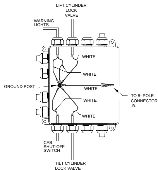
GROUND WIRE CONNECTIONS
