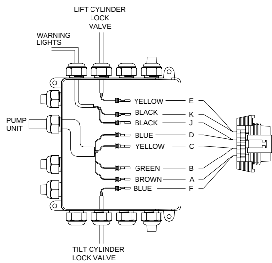
10- POLE CONNECTOR
